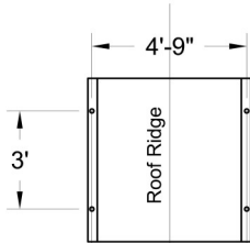
Plan View A-A
