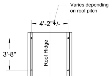
Plan View A-A Scale: 3/16" = 1'-0"
