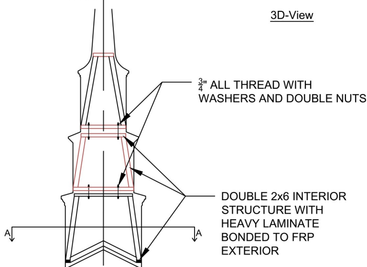
Interior Support Detail Scale: 1/8" = 1'-0"
