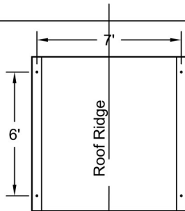
Plan View A-A Scale: 3/16" = 1'-0"
