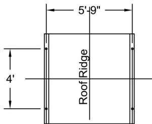
Plan View A-A Scale: 3/16" = 1'-0"
