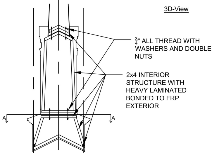
Interior Support Detail Scale: 3/16" = 1'-0"
