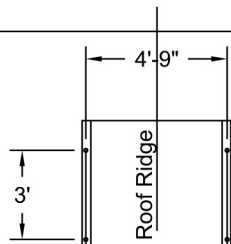
Plan View A-A Scale: 3/16" = 1'-0"
