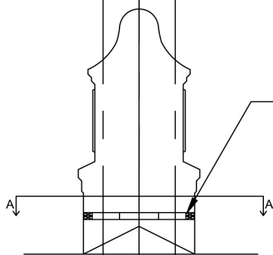
Interior Support Detail Scale: 1/4" = 1'-0"
