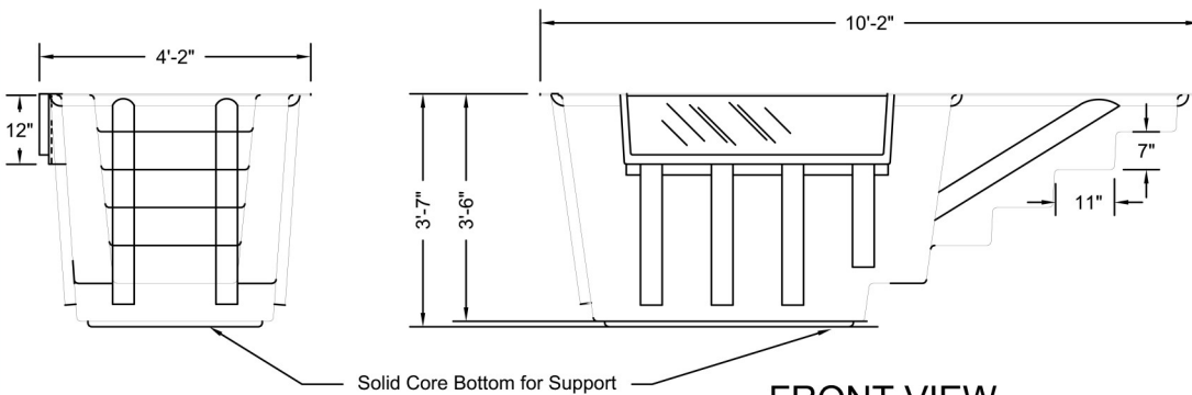
FRONT VIEW
