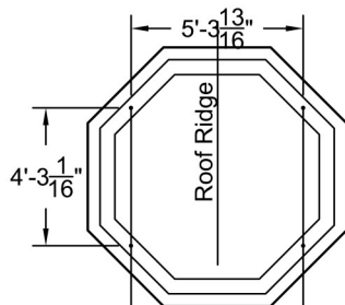
Plan View A-A Scale: 3/16" = 1'-0"
