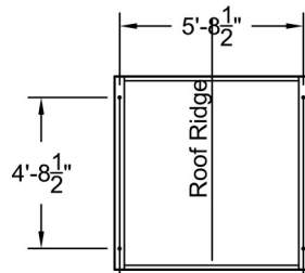
Plan View A-A Scale: 3/16" = 1'-0"
