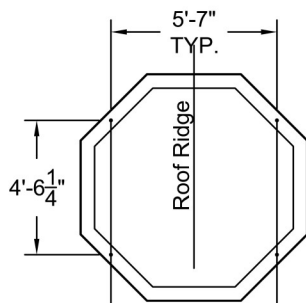
Plan View A-A Scale: 3/16" = 1'-0"
