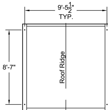
Plan View A-A Scale: 3/16" = 1'-0"
