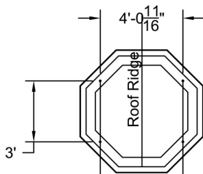
Plan View A-A Scale: 3/16" = 1'-0"
