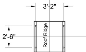
Plan View A-A Scale: 3/16" = 1'-0"
