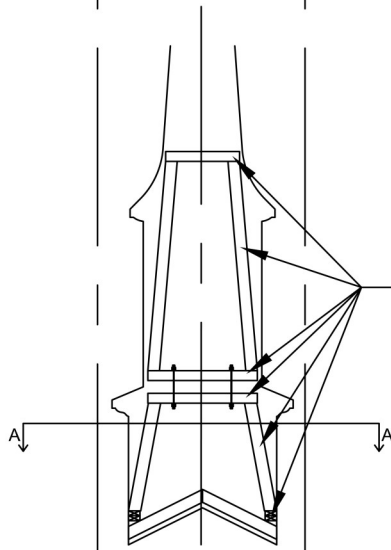
Interior Support Detail Scale: 1/4" = 1'-0"
