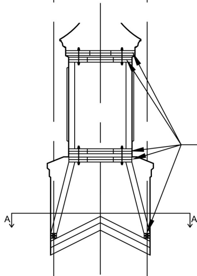
Interior Support Detail Scale: 1/4" = 1'-0"
