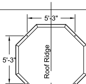
Plan View A-A Scale: 3/16" = 1'-0"
