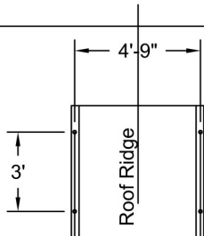
Plan View A-A Scale: 3/16" = 1'-0"
