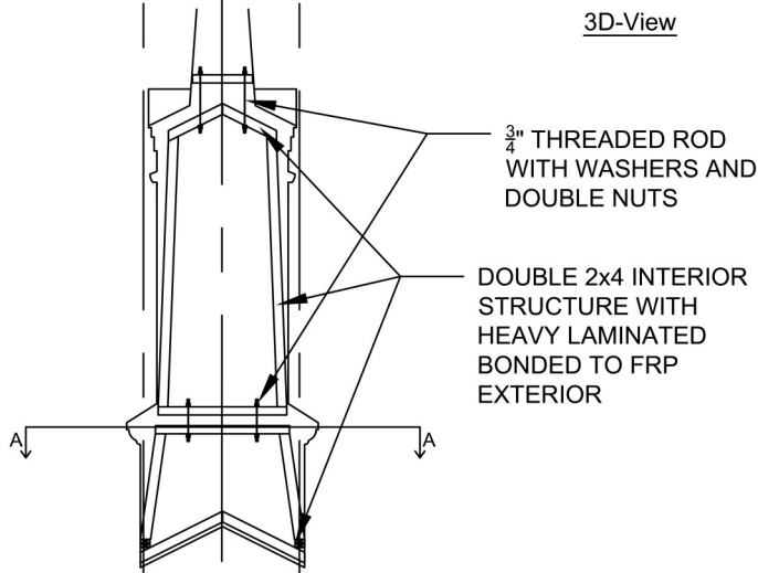
Interior Support Detail Scale: 3/16" = 1'-0"
