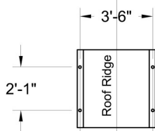
Plan View A-A Scale: 3/16" = 1'-0"
