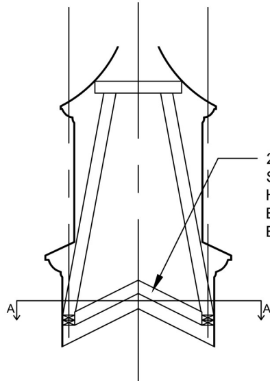
Interior Support Detail Scale: 3/8" = 1'-0"
