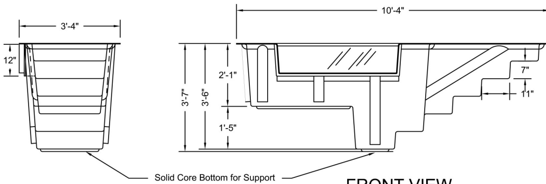
FRONT VIEW
