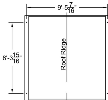
Plan View A-A Scale: 3/16" = 1'-0"
