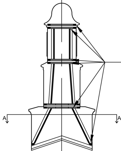
Interior Support Detail Scale: 1/4" = 1'-0"
