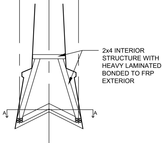
Interior Support Detail Scale: 3/8" = 1'-0"
