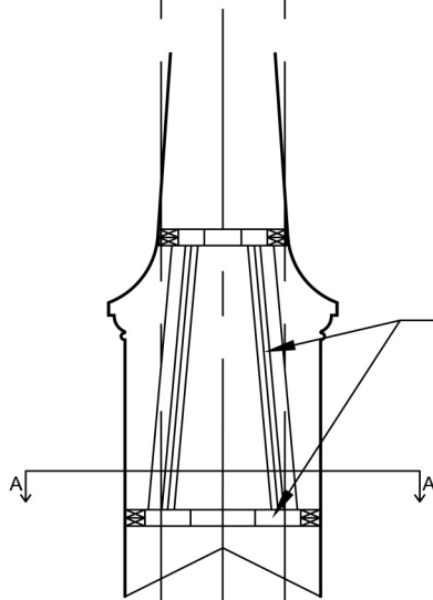
Interior Support Detail Scale: 3/8" = 1'-0"
