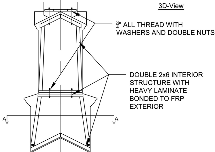
Interior Support Detail
