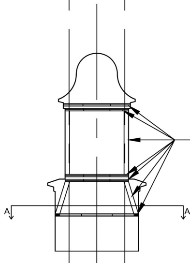
Interior Support Detail Scale: 1/8" = 1'-0"
