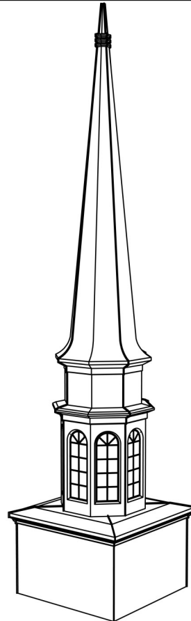
3D-View
