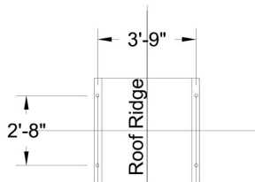
Plan View A-A Scale: 3/16" = 1'-0"
