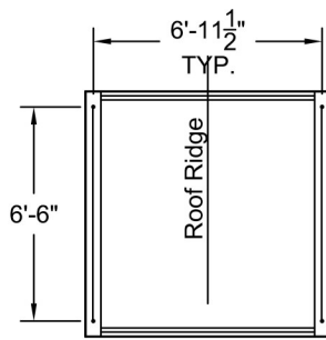
Plan View A-A Scale: 3/16" = 1'-0"
